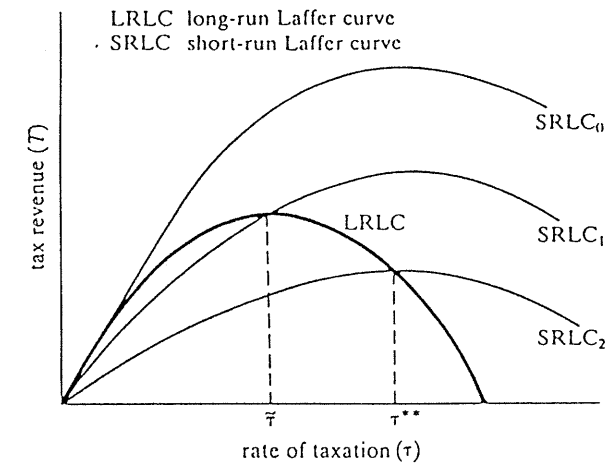
Figure 6.1 Short-run and long-run Laffer curves, the equilibrium rate of taxation ( \tau^{**} ) and the long-run revenue-maximizing rate of taxation ( \bar{\tau} ).
